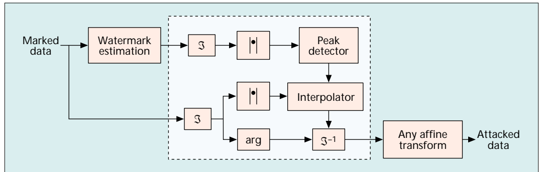
■ Figure 3. A synchronization removal attack.
